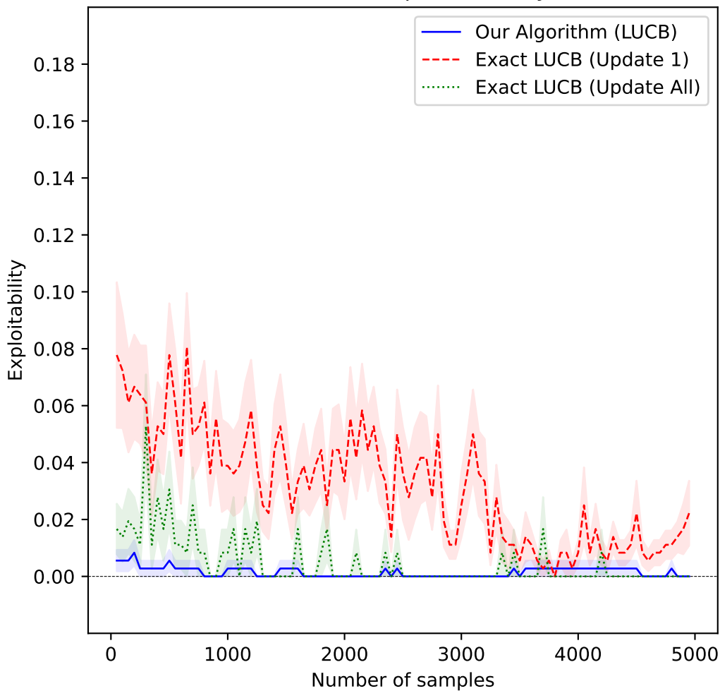
Kuhn Poker, Comparison, Player x
